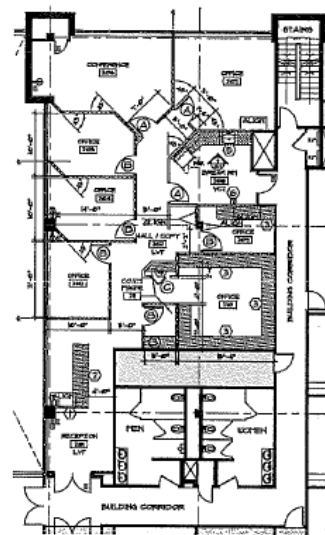
2nd FLOOR
